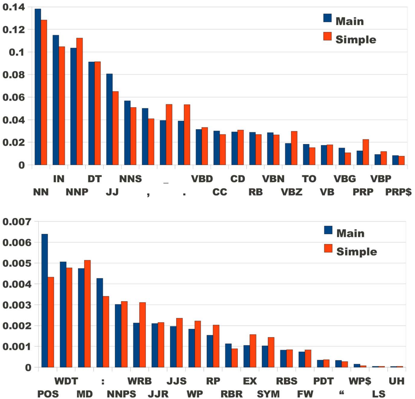
Figure 3. Part of Speech statistics of Main English and Simple English Wikipedias. Condition O, as explained in the Methods section. The legends are defined as NN: Noun, singular or mass; IN: Preposition or subordinating conjunction; NNP: Proper noun, singular; DT: Determiner; JJ: Adjective; NNS: Noun, plural; VBD: Verb, past tense; CC: Coordinating conjunction; CD: Cardinal number; RB: Adverb; VBN: Verb, past participle; VBZ: Verb, 3rd person singular present; TO: to; VB: Verb, base form; VBG: Verb, gerund or present participle; PRP: Personal pronoun; VBP: Verb, non-3rd person singular present; PRP$: Possessive pronoun; POS: Possessive ending; WDT: Wh-determiner; MD: Modal; NNPS: Proper noun, plural; WRB: Wh-adverb; JJR: Adjective, comparative; JJS: Adjective, superlative; WP: Wh-pronoun; RP: Particle; RBR: Adverb, comparative; EX: Existential there; SYM: Symbol; RBS: Adverb, superlative; FW: Foreign word; PDT: Predeterminer; WP$: Possessive wh-pronoun; LS: List item marker; UH: Interjection. doi:10.1371/journal.pone.0048386.g003
